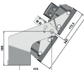
Picture shows variant flood light FU
